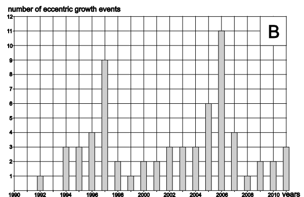
Fig. 10. The number of debris flow events recorded by tree-ring analyses, (A) – results of the dating of wounded alder stems, (B) – results of the dating using eccentric growth.
