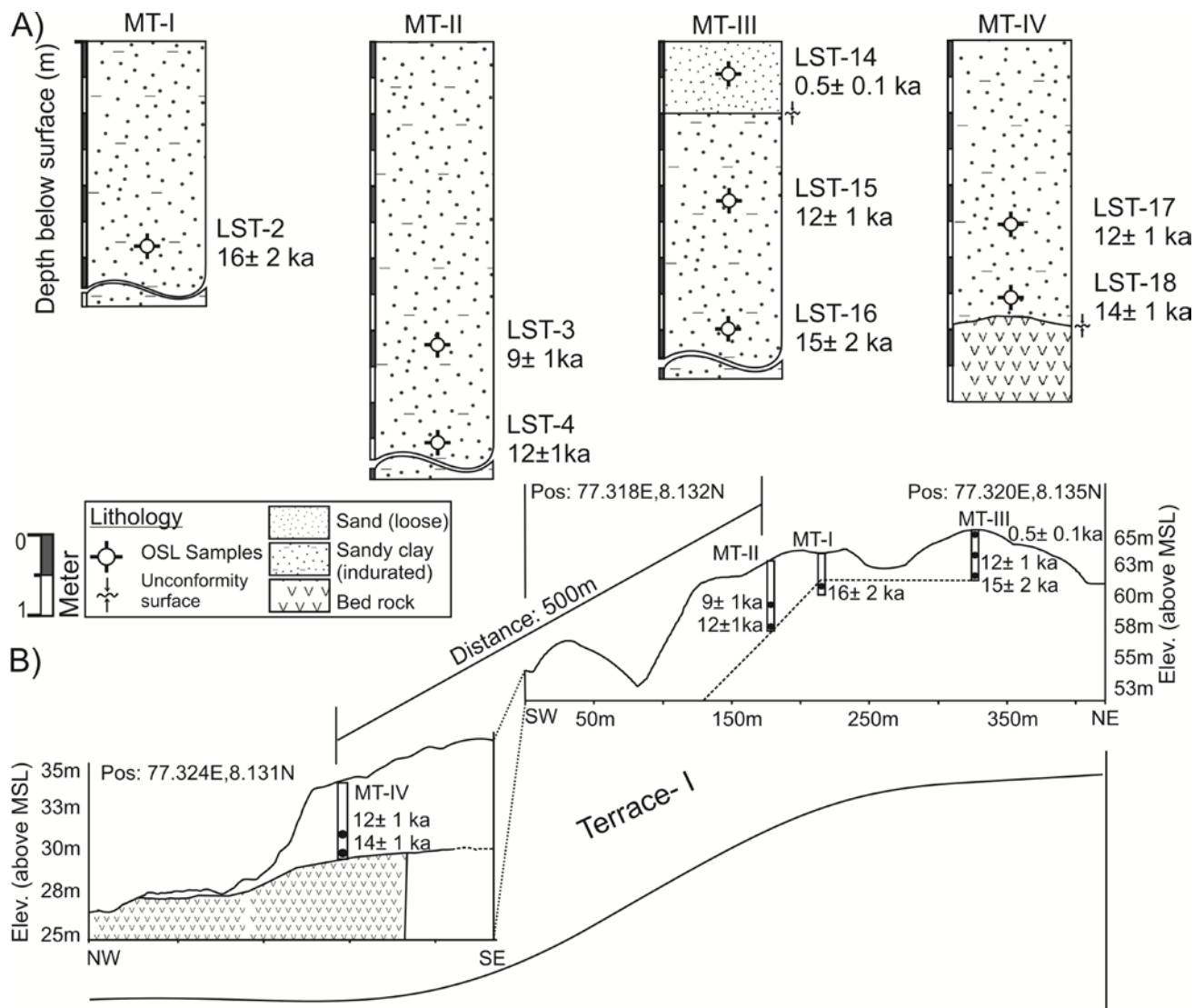
Fig. 2. A) Illustrations showing the stratigraphic succession in the excavated dune sections at Muttom along with OSL sample positions and ages, B) showing the overall view and elevation of the dune field in the transect, where different sections are located.
